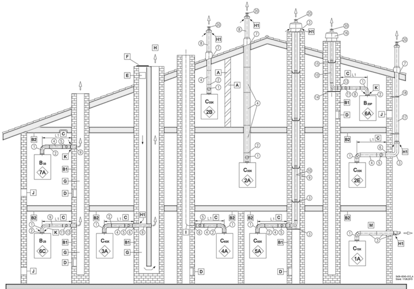
Abb. 22: Installationsarten
